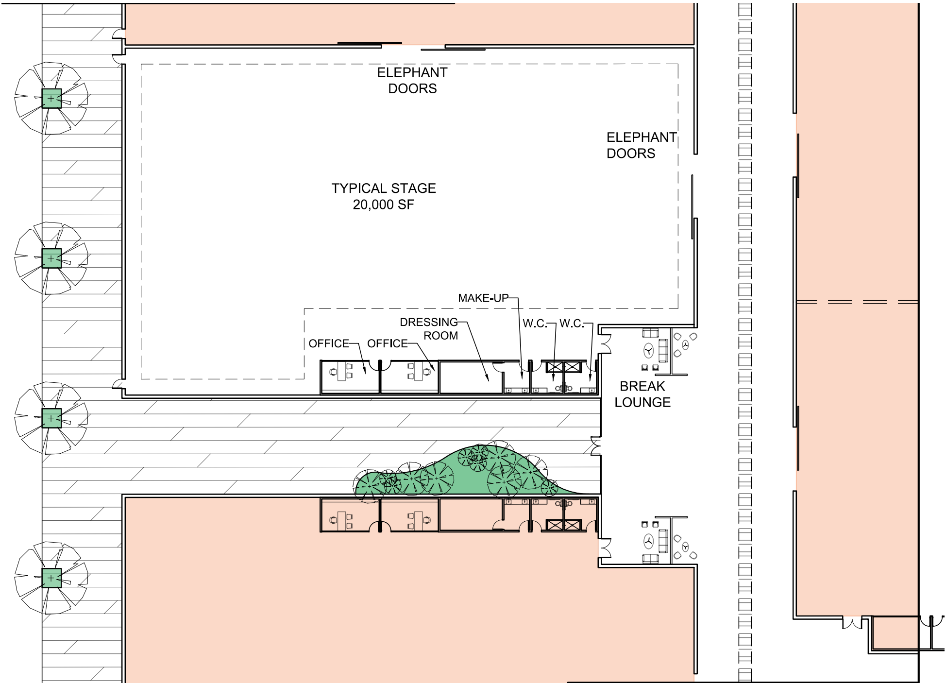
TYPICAL STAGE FLOOR PLAN
