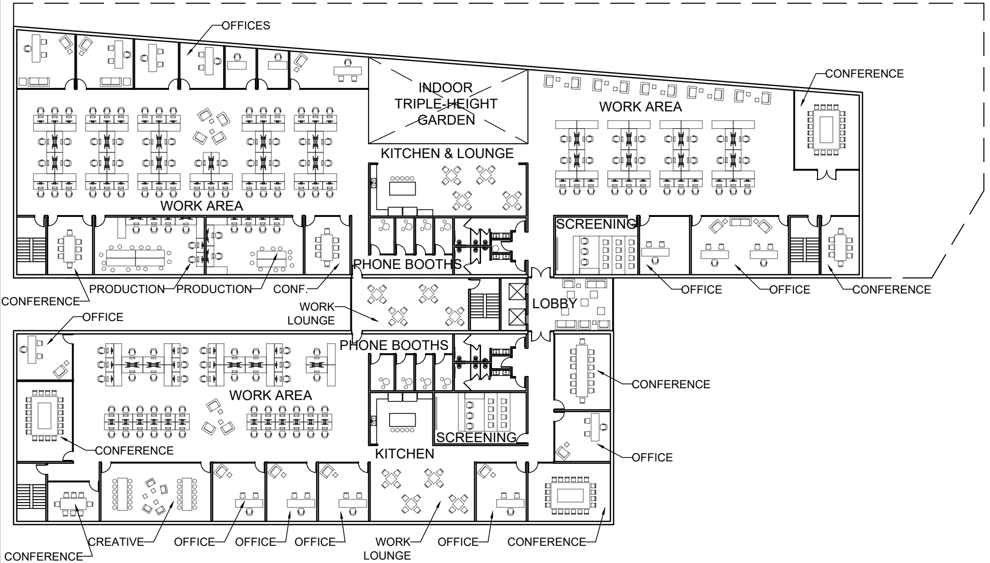
TYPICAL OFFICE FLOOR PLAN
